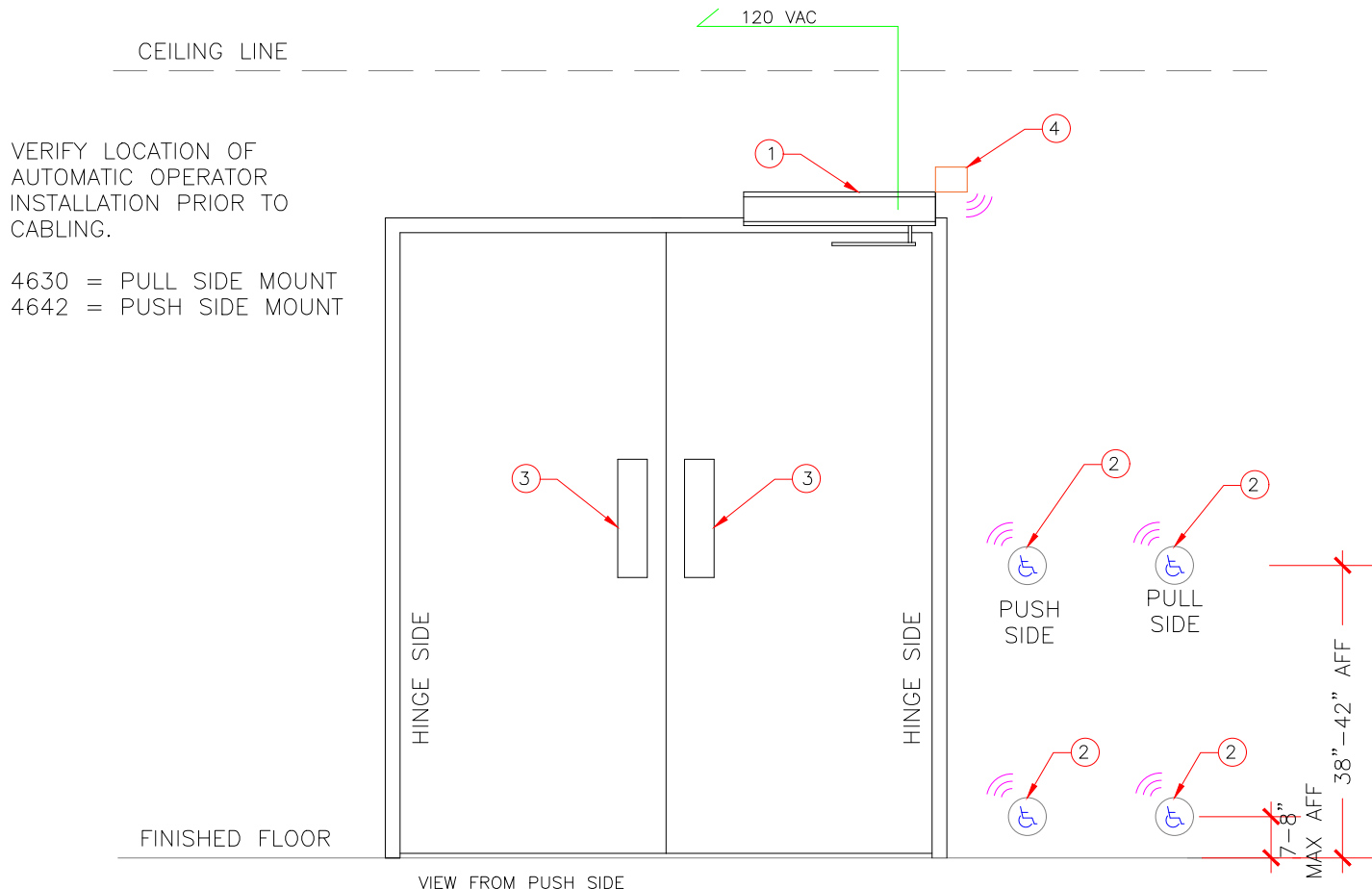
VIEW FROM PUSH SIDE
