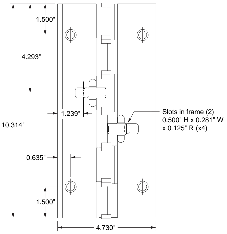
Vertical distance between holes (120" length shown)
