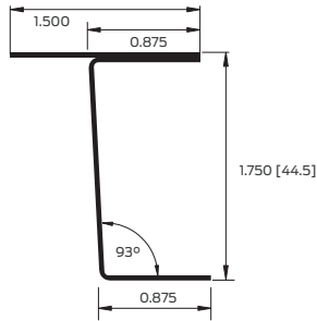
7302B-A (mortised)
