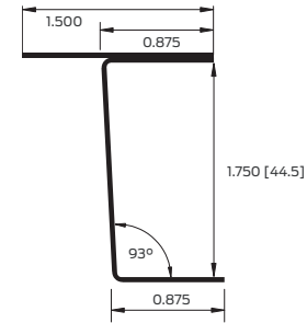
7306B-A (non-mortised)
