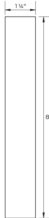
No. 5 Mortise lock cutout
