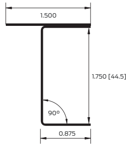
7306-A (non-mortised)
