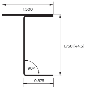
7302-A (mortised)
