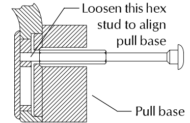
Figure 3. Tighten thru bolt in pull base.
