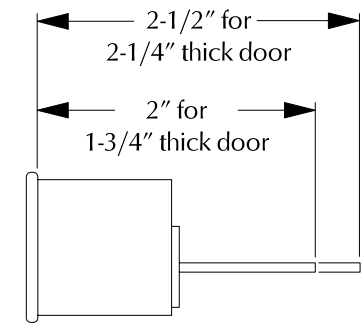
Figure 2. Cut cylinder tailpiece to length.
