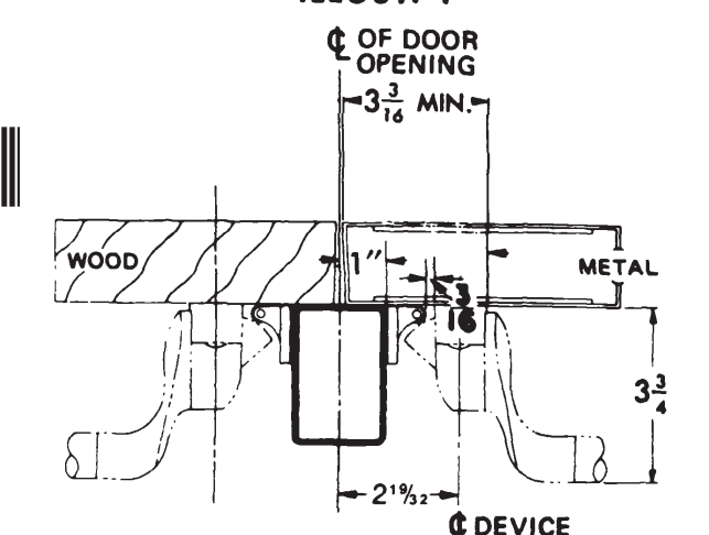
ILLUST. 2 4954 MULLION WITH 299 STRIKE
