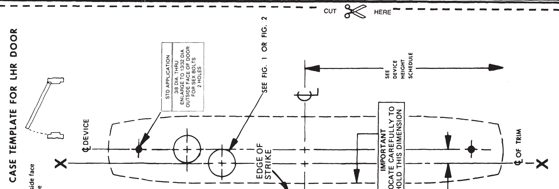
LOCK CASE TEMPLATE FOR LHR DOOR
