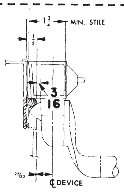
ILLUS. 6 1410 STRIKE SINGLE DOOR NARROW STILE
