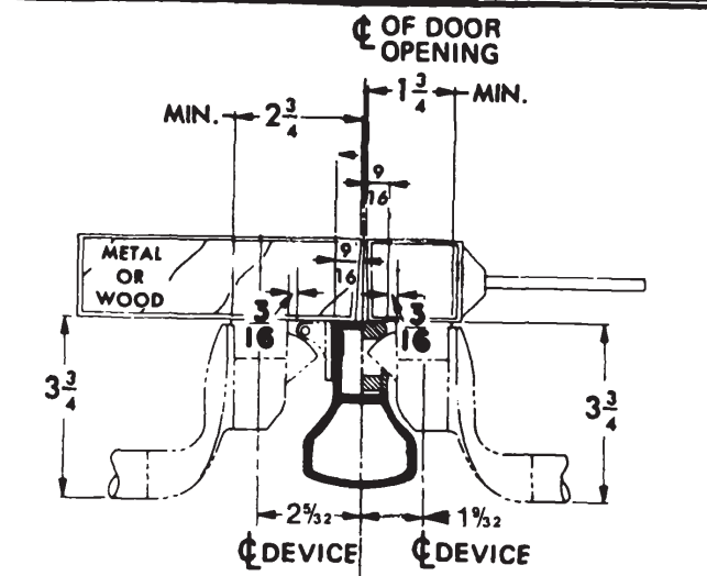
ILLUST. 1 5254 OR 5654 MULLION WITH 299 STRIKE 5554 OR 5754 MULLION WITH 1408 STRIKE
