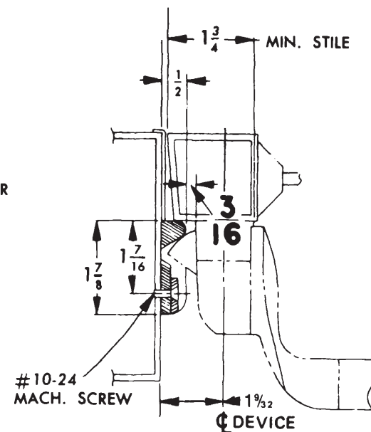
ILLUST. 4 1409 STRIKE SINGLE DOOR NARROW STILE
