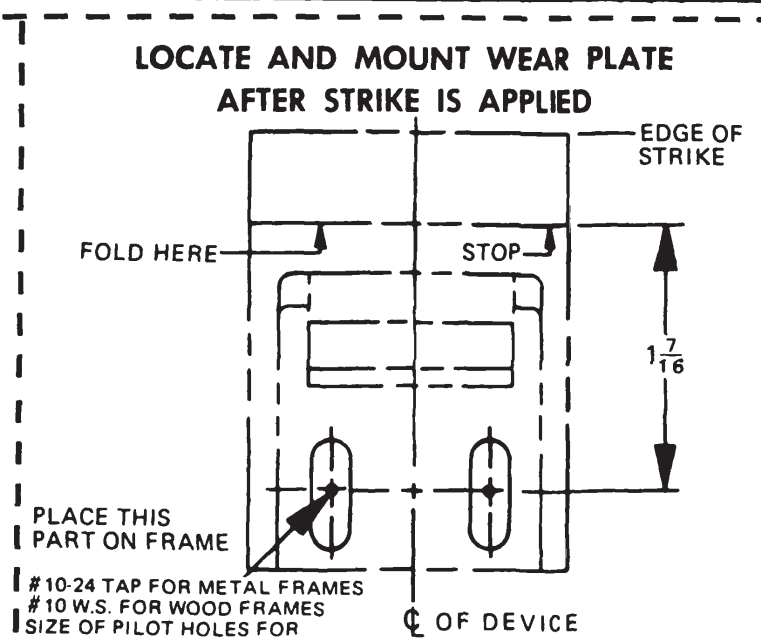
1409 STRIKE TEMPLATE NO. 3
