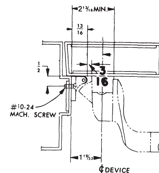
299 STRIKE SINGLE DOOR WIDE STILE ILLUST. 5
