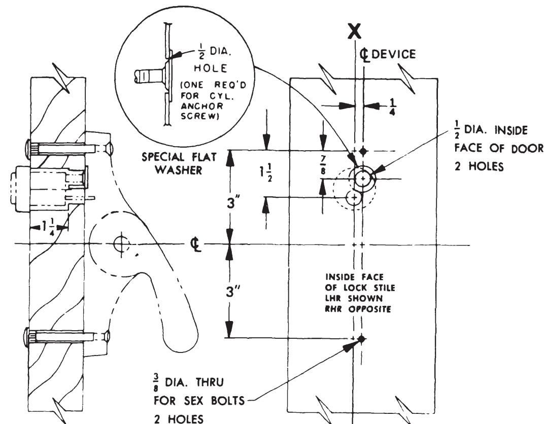
WOOD DOOR APPLICATION FIG. 1
