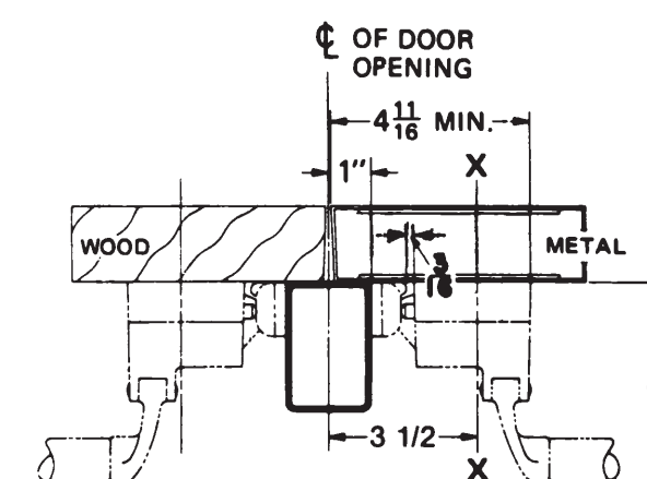
ILLUST. 1 9954 MULLION WITH 268 STRIKE
