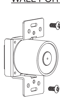
Magnet Bracket Assembly
