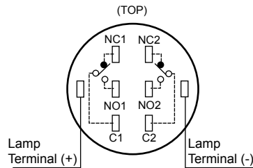
DPDT Contact (Double-pole/Double Throw)
