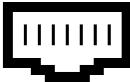
Figure 12-5: J4 - RJ-45/RS-232 Jack Pinout
