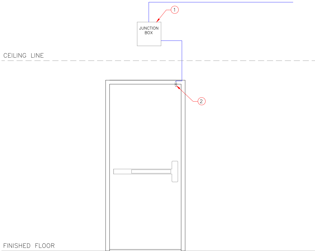
DOOR ELEVATION – DOOR MONITOR ONLY N.T.S.
