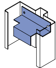
"Z" Anchor (Optional) Must be welded in
