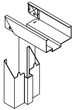
ME Corner Connection
